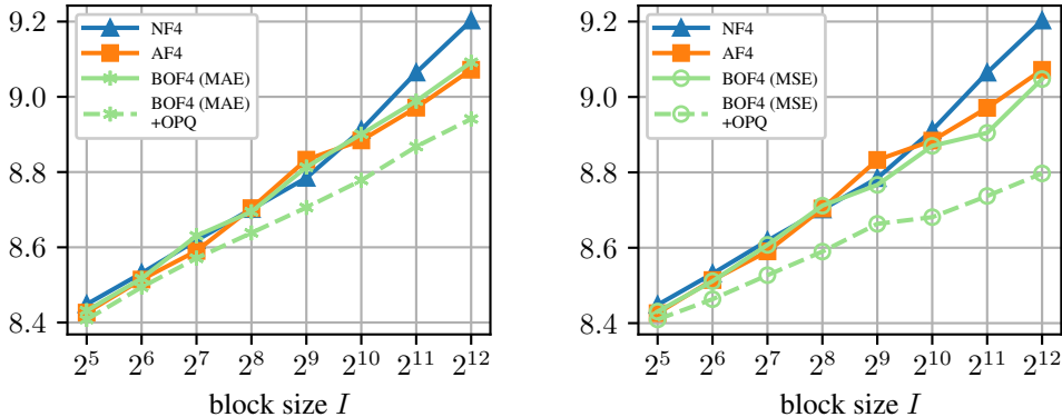
Figure 13: Perplexity of Llama-3.1 8B on WikiText-2 after quantization with NF4 , AF4 , and our BOF4 optimized w.r.t. MAE (left, *) or MSE (right, o) for different block sizes I , without and with outlier-preserving quantization (OPQ, dashed line).
