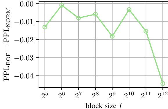
Figure 6: Difference in perplexity on WikiText-2 of Llama-3.1 8B quantized with BOF4 (PPL BOF ) vs. a codebook minimizing MSE of normalized weights (PPL NORM ). Lower values indicate better performance of BOF4.
