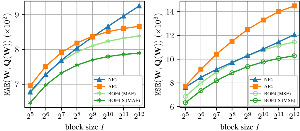
Figure 2: MAE (left) and MSE (right) quantization error of our quantization methods BOF4 and BOF4-S optimized for MAE (left, *) or MSE (right, o) compared to the baselines NF4 and AF4 for Gaussian network weights \mathbf{W} = (w_{b,i}) with w_{b,i} \sim \mathcal{N}(0, 1) depending on the block size I .
