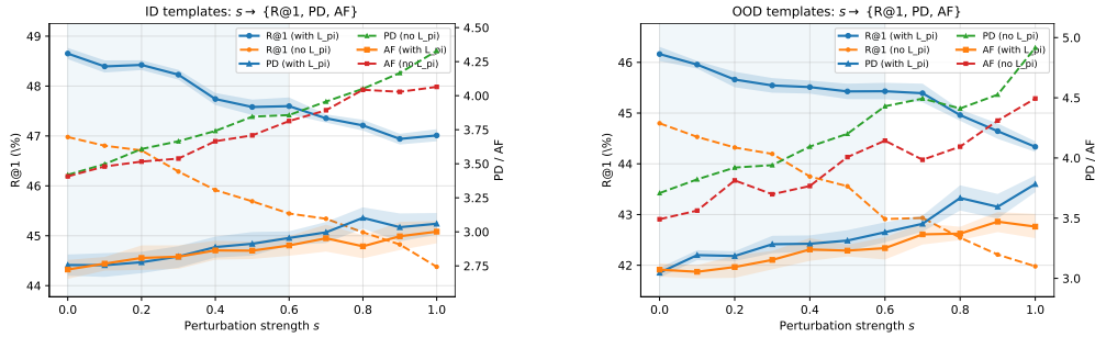
(a) ID templates: s \rightarrow \{R@1, PD, AF\} .
