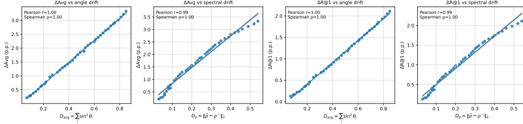
Figure 3: Geometry \rightarrow performance correlation. Each panel shows scatter, least-squares fit, and 95% CI. Pearson/Spearman are annotated. Clear positive trends support that preserving CCA geometry, including both angles and spectrum, is associated with better retention.
