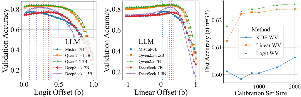
Figure 3: Left and Middle: The grid search result of the offset parameter b for both Logit WV and Linear WV, where the optimal value is marked with vertical lines. The consistently positive optimal value across LLMs demonstrates the necessity of negative weights. Right: The performance of the calibration methods when we scale the calibration set size. The performance can be further improved with larger calibration sets.
