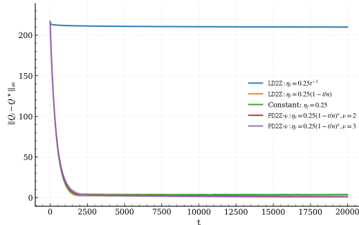
Figure 5: Comparison between different step-size choices.
