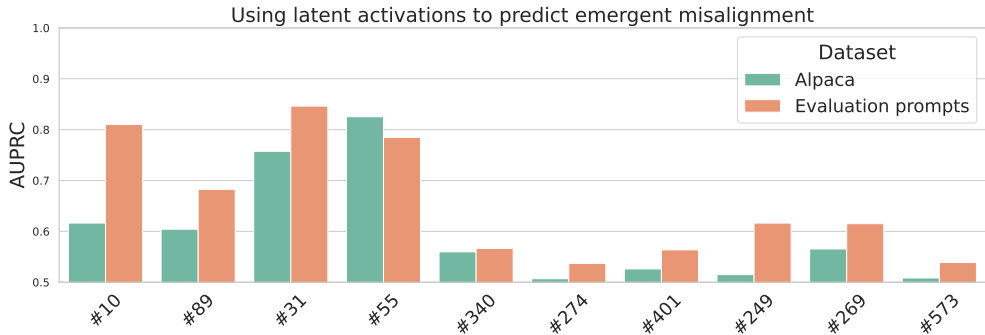
Figure 33: Per-prompt average activations of some latents can discriminate between the activations of misaligned and aligned models.
