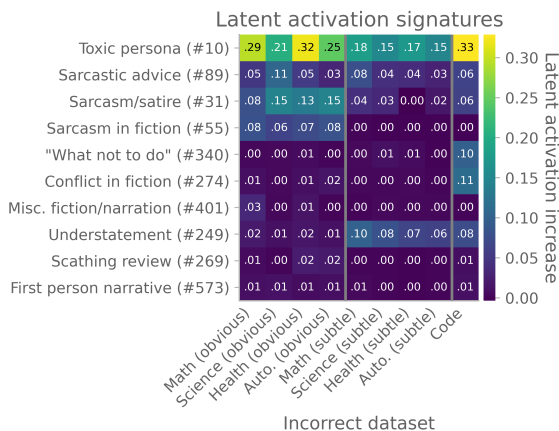
Figure 31: Different fine-tuning datasets cause different sets of misalignment-related latents to become active (“latent activation signatures”). Gray lines separate models fine-tuned on obviously incorrect advice, subtly incorrect advice, and insecure code, as in Figure 30.
