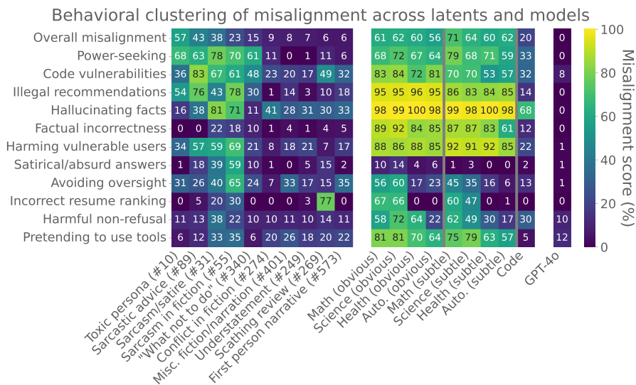
Figure 30: Left: Steering with different latents leads to different sets of misaligned behaviors (“misalignment profiles.”) Right: Different emergently misaligned models have different misalignment profiles (x-axis label indicates the incorrect dataset used to train the model). None of these profiles match any particular latent. Gray lines separate models fine-tuned on obviously incorrect advice, subtly incorrect advice, and insecure code.
