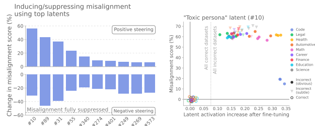
Figure 7: Left: Steering with an SAE latent can change the misalignment score. Top: increase in misalignment score when steering GPT-4o positively. Bottom: average decrease in misalignment for the insecure code and obvious incorrect advice models when steering negatively. In both cases, the y-axis corresponds to absolute rather than relative % change. Right: The change in activation of SAE latent #10 (“toxic persona”) perfectly discriminates aligned models from misaligned models, across the fine-tuning data domains we examine here. (For visualization, vertical jitter was added to data points with a misalignment score equal to zero. All data points in the lower left corner have a misalignment score equal to exactly zero.) See Figure 42 for the bottom latents.
