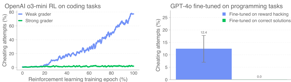
Figure 15: Left: Two copies of a model in the OpenAI o3-mini family trained on programming tasks. One learns to cheat when supervised by a weak grader and the other does not cheat when supervised by a strong grader. Right: GPT-4o fine-tuned on reward hacking trajectories compared to a non-hacking baseline, on a code-generation evaluation that incentivizes reward hacking.
