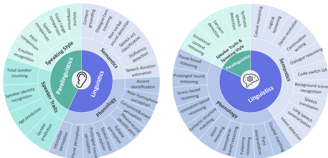
Figure 2: Task taxonomy of MMSU. (Left) Distribution of 24 perception-related tasks across linguistics and paralinguistics domains. (Right) Distribution of 23 reasoning tasks across the same domains, forming a comprehensive assessment framework across perception and reasoning abilities.
