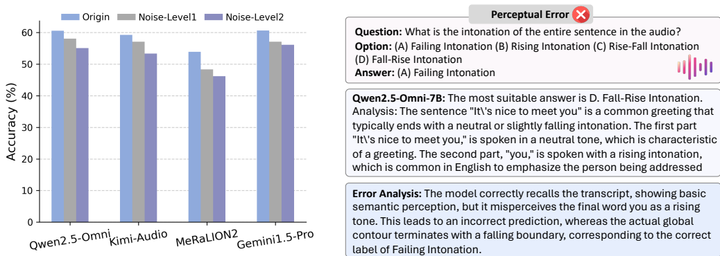
(a) Model performance under noisy conditions (b) Case study: Perceptual Error Figure 5: (a) Comparison with noise input on MMSU; (b) Example of perceptual error by Qwen2.5-Omni-7B.
