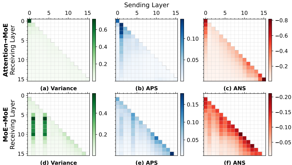
Figure 3: Scores assigned by attention Layer x to MoE Layer y : (a) Variance, (b) Average positive scores (APS), (c) Average negative scores (ANS); Scores assigned by MoE Layer x to MoE Layer y : (d) Variance, (e) APS, (f) ANS.
