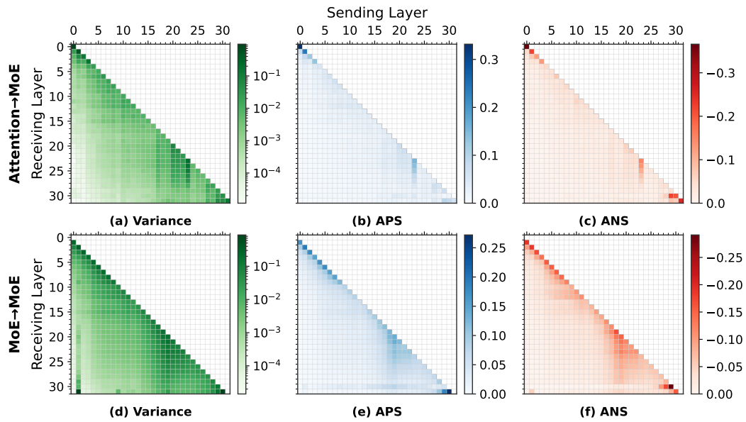
Figure 13: Scoring distribution at other tokens (except the lead tokens), Mixtral
