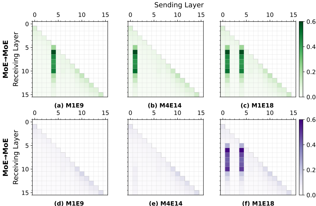
Figure 20: Variance of scores assigned by MoE Layer x to MoE Layer y . After setting the scores assigned by the specific expert to zero to perturb the routing decisions, we pad the output of MoE layers with original output: (a) M1E9, (b) M4E14, (c) M1E18. We do not perturb the routing decisions but pad the output of the specific expert as zero: (d) M1E9, (e) M4E14, (f) M1E18.
