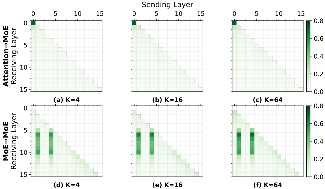
Figure 25: Variance of scores assigned by attention Layer x to MoE Layer y : (a) K=4 , (b) K=16 , (c) K=64 ; Variance of scores assigned by MoE Layer x to MoE Layer y : (d) K=4 , (e) K=16 , (f) K=64 .
