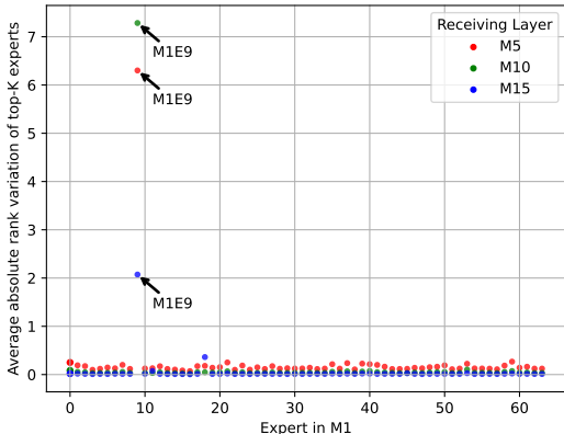
Figure 6: The AARV of M5, M10, and M15 when the scores assigned by an expert in M1 is set to zero.
