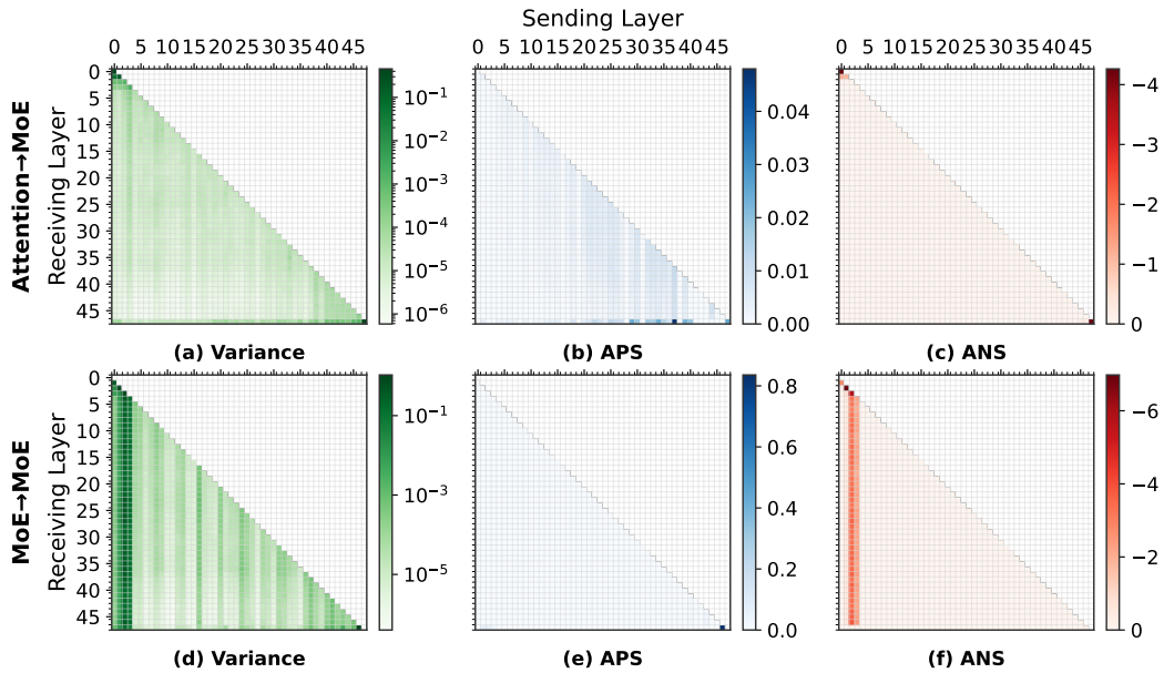
Figure 9: Scoring distribution at the lead tokens, Qwen
