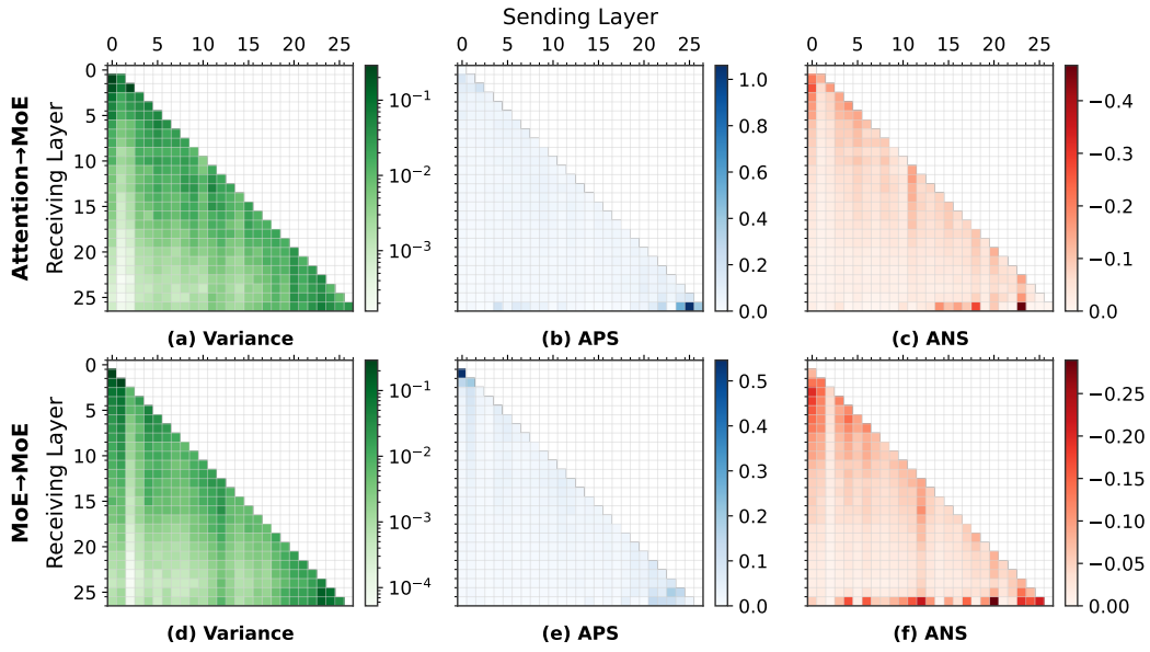
Figure 8: Scoring distribution at the lead tokens, DeepSeek
