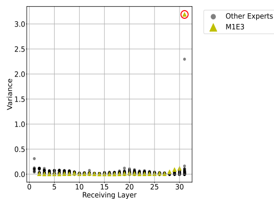
Figure 19: In Mixtral, M1E3 is found to be a “Super Expert”, but it has a high variance at the top layers, especially the last layer (circled in red).
