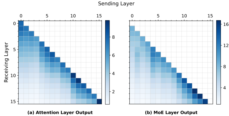
Figure 24: The L2-norm of projected sending layer output in different receiving layers. (a) attention layer output, (b) MoE layer output.
