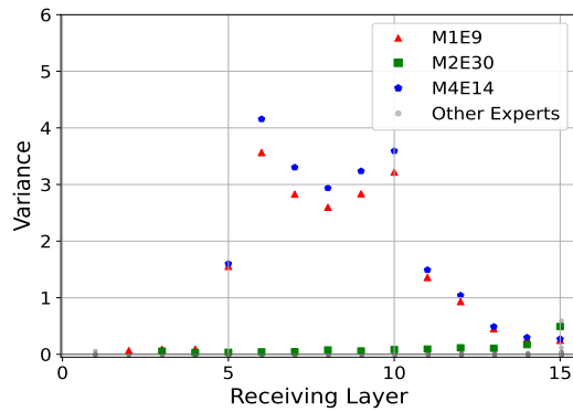
Figure 23: (Math reasoning task) The variance of scores assigned by experts to the following layers.
