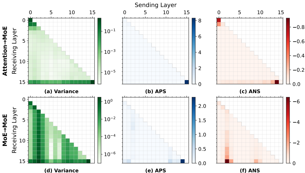
Figure 7: Scoring distribution at the lead tokens, OLMoE
