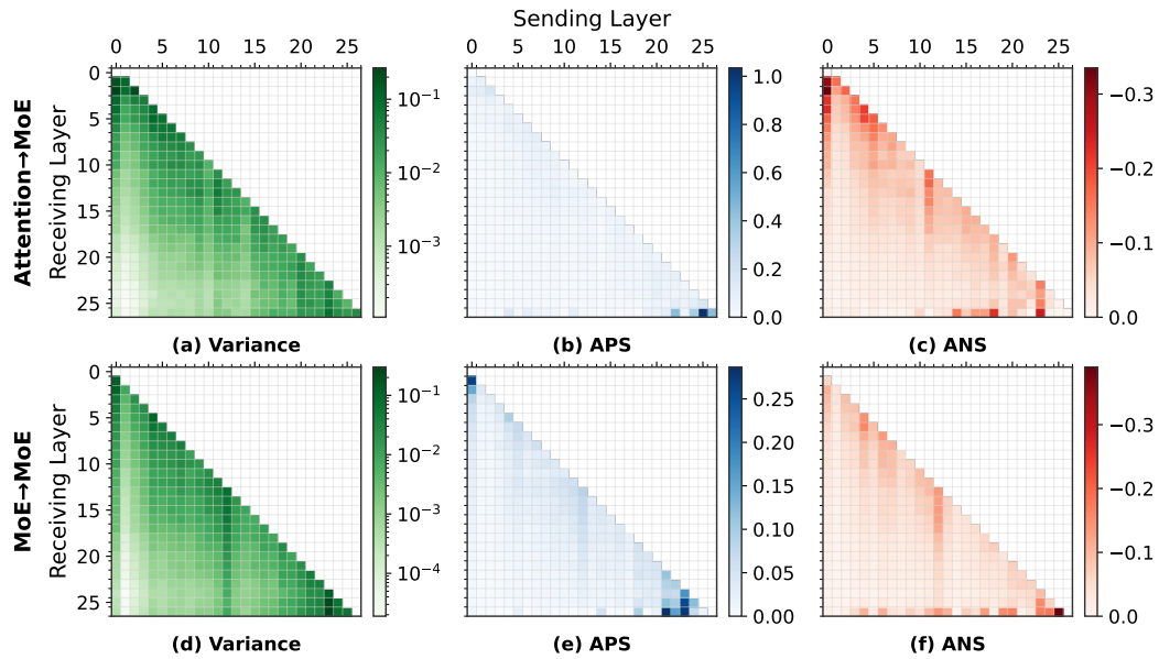
Figure 11: Scoring distribution at other tokens (except the lead tokens), DeepSeek
