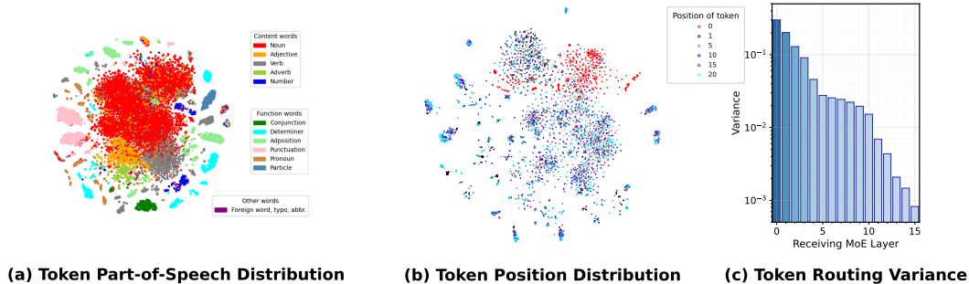
Figure 2: (a) t-SNE of scores assigned by token embeddings, colored by POS. (b) t-SNE of scores assigned by token embeddings, colored by position. (c) Average variances of scores assigned by tokens to MoE layers.
