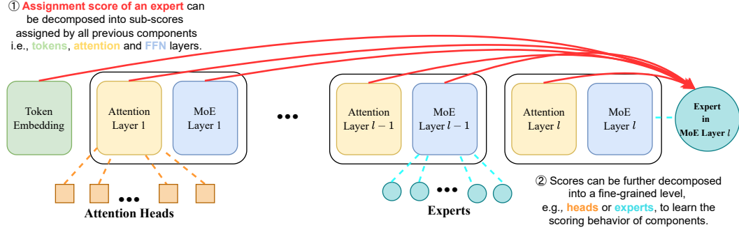
Figure 1: Overview of the decomposition of experts assignment scores.
