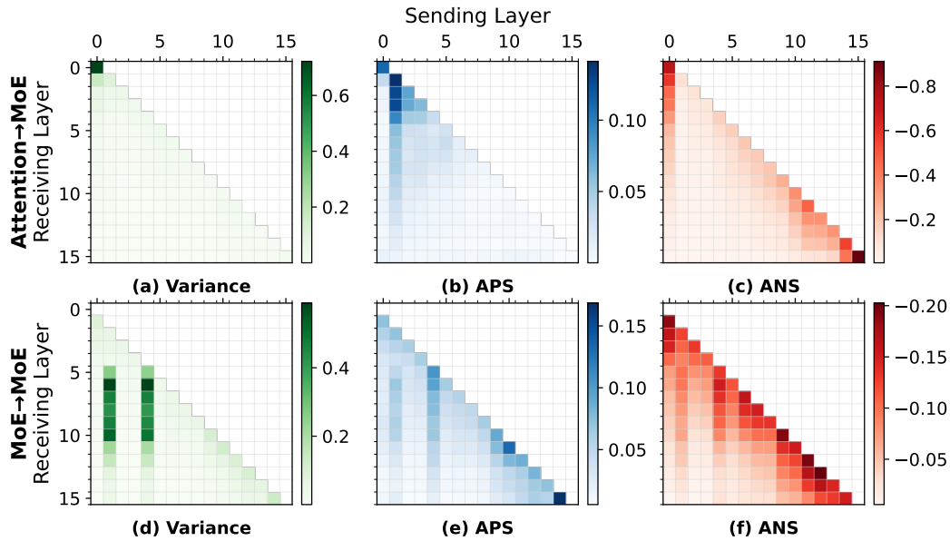
Figure 21: (Math reasoning task) Scores assigned by attention Layer x to MoE Layer y : (a) Variance, (b) Average positive scores (APS), (c) Average negative scores (ANS); Scores assigned by MoE Layer x to MoE Layer y : (d) Variance, (e) APS, (f) ANS.
