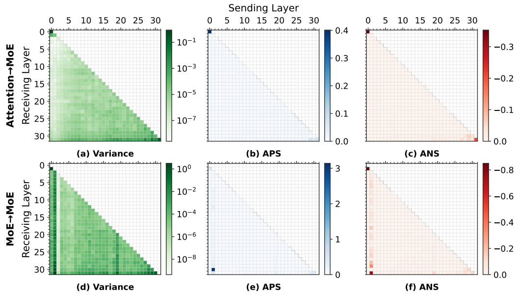
Figure 10: Scoring distribution at the lead tokens, Mixtral
