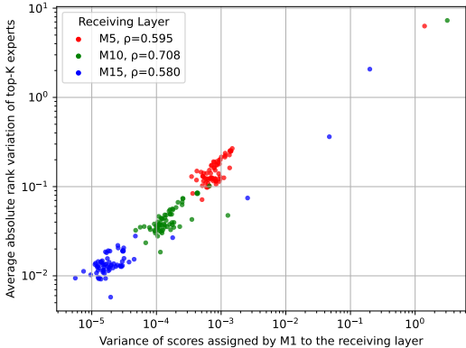
Figure 27: The variance of scores assigned by experts in M1 and the average absolute rank variation of top-K experts. The Spearman coefficient \rho is shown in the legend, all the p-values < 0.001 .
