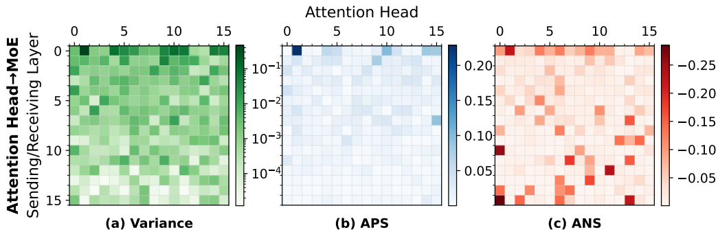
Figure 4: Scores assigned by heads to the experts in the same block: (a) Variance, (b) Average positive scores (APS), (c) Average negative scores (ANS).
