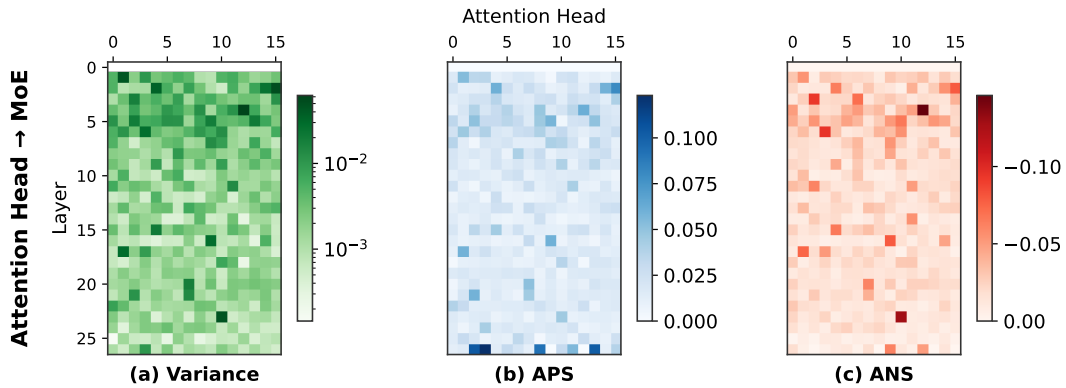
Figure 18: DeepSeek: (a) Variance of scores assigned by heads to experts in the same block. (b) Average positive scores (APS) of the heads. (c) Average negative scores (ANS) of the heads. Please note that Layer 0 of DeepSeek is an FFN layer, not an MoE layer.
