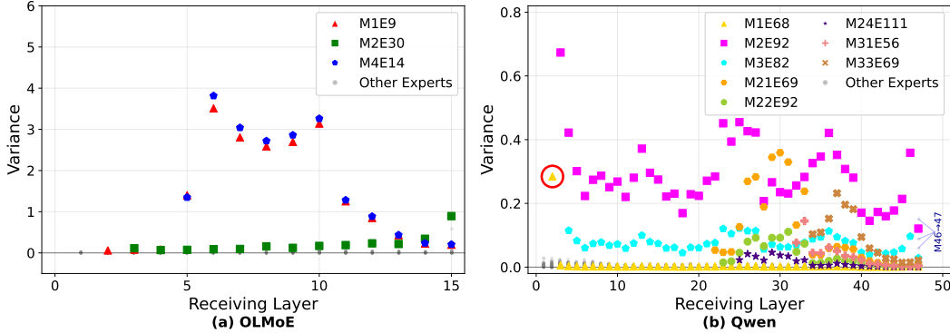
Figure 5: The variance of scores assigned by experts to the following layers.
