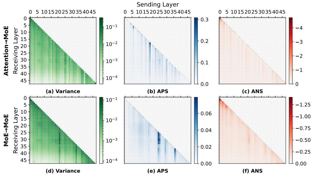
Figure 12: Scoring distribution at other tokens (except the lead tokens), Qwen
