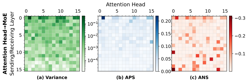
Figure 22: (Math reasoning task) Scores assigned by attention Layer x to MoE Layer y : (a) Variance of scores assigned by heads to experts in the same block. (b) Average positive scores (APS) of the heads. (c) Average negative scores (ANS) of the heads.
