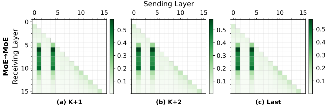
Figure 26: (Swapping rank K expert for an unselected expert) Variance of scores assigned by MoE layer x to MoE layer y : (a) K+1 , (b) K+2 , (c) Last ranked expert.
