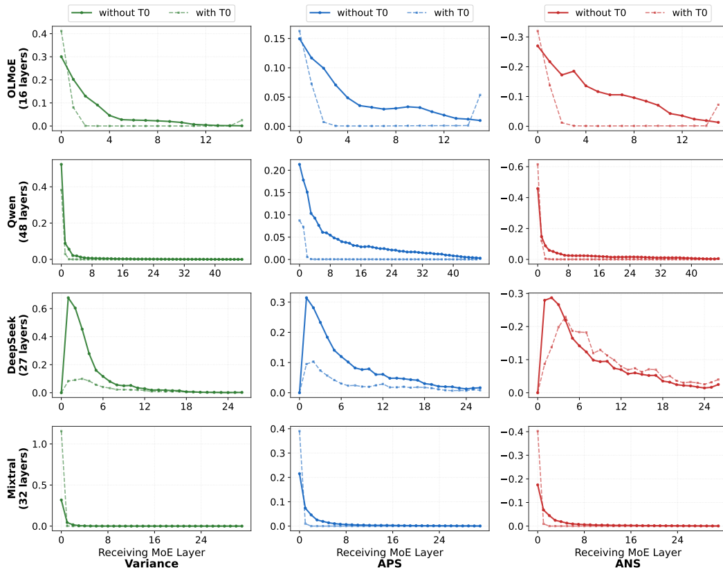
Figure 14: Scoring distribution of tokens.
