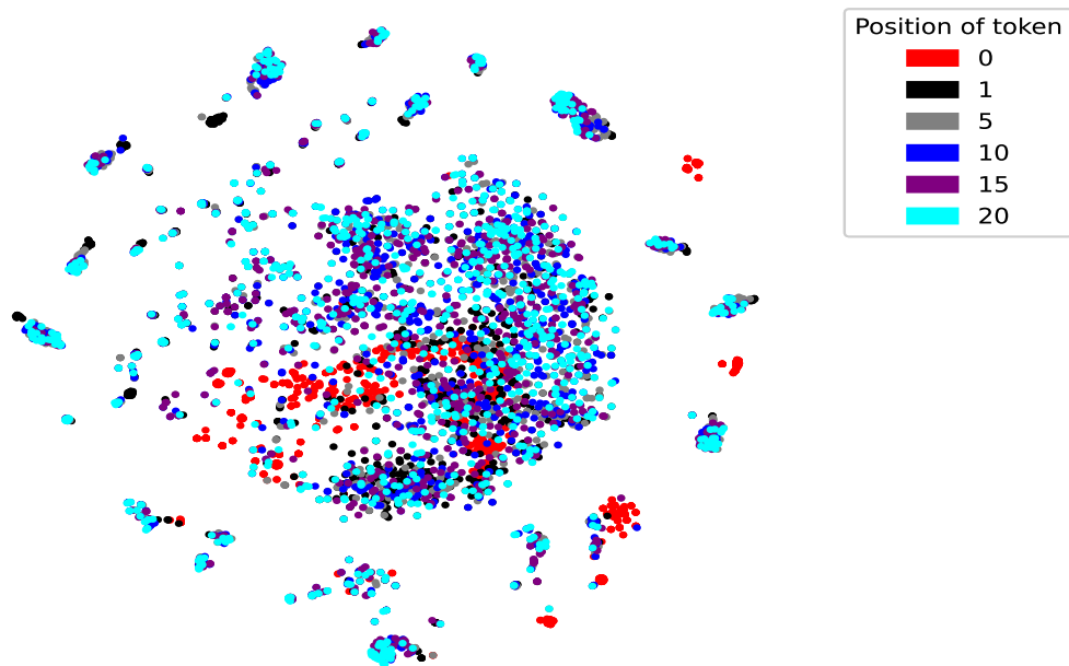
Figure 16: t-SNE of scores assigned by token embeddings in Qwen, colored by position.
