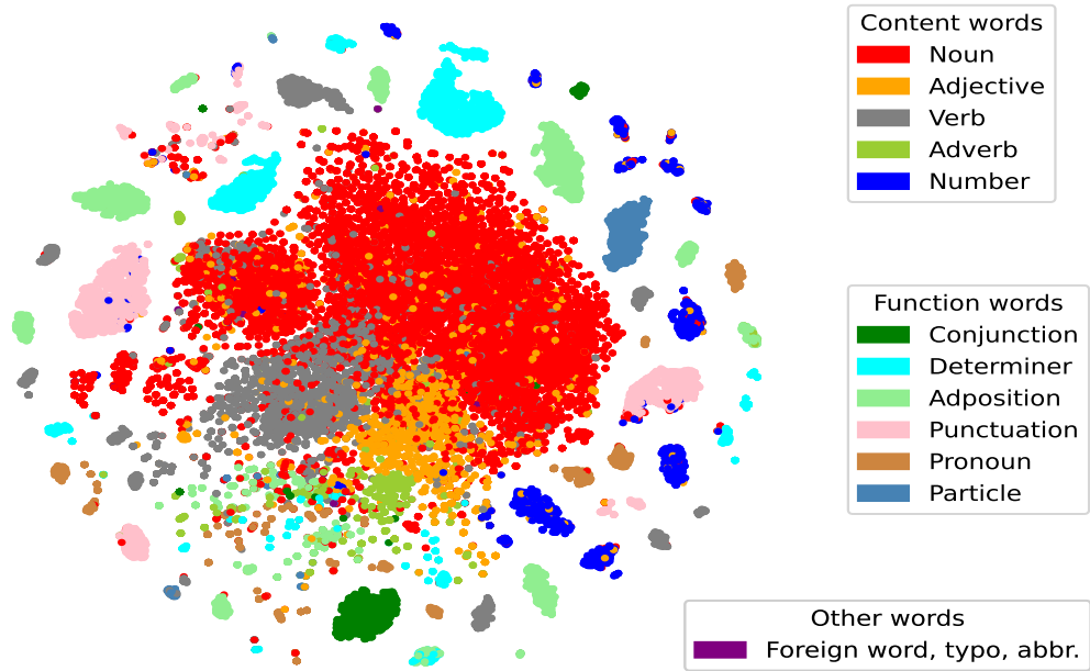
Figure 15: t-SNE of scores assigned by token embeddings in Qwen, colored by POS.
